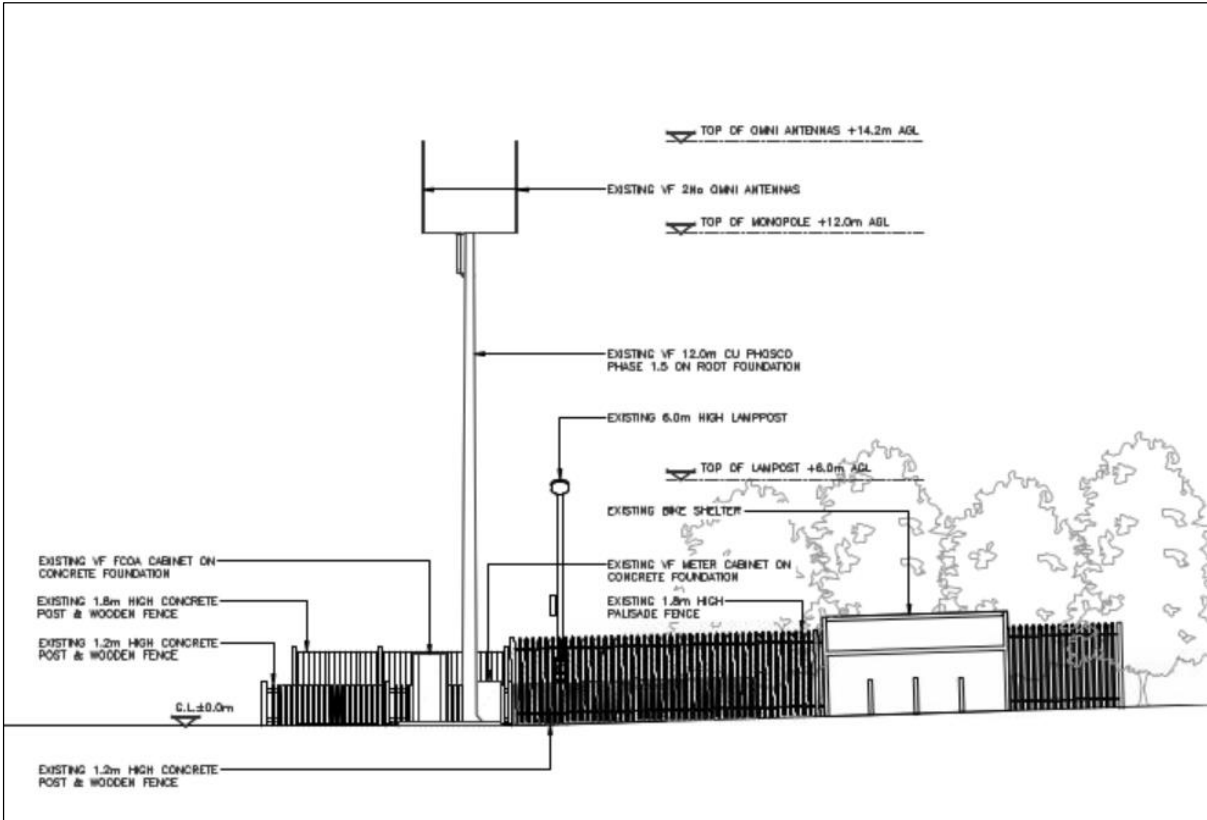
Existing site elevation
