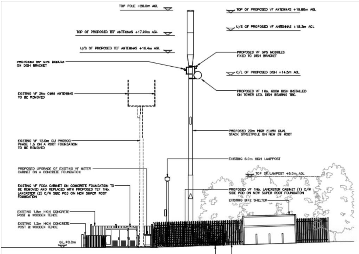
Proposed site elevation
