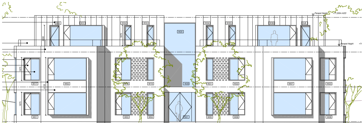
Proposed front elevation (North-east)
